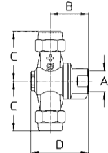
73.605.27 G3/8 3/8" BSPF
